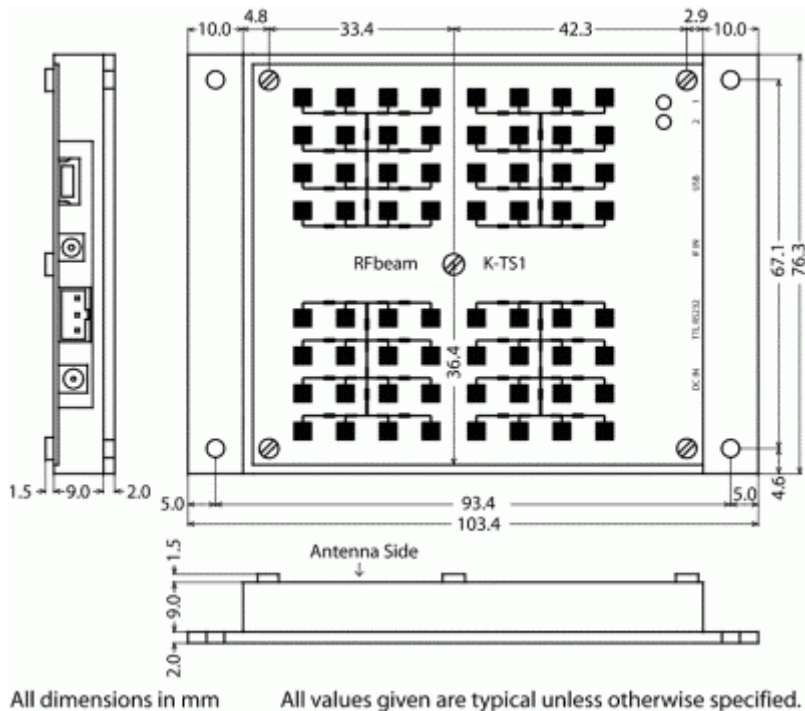
Fig. 13: Mechanical dimensions
