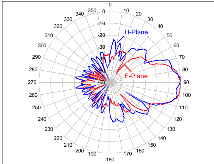
Fig. 3: Field Pattern of Tx Antenna
