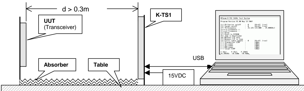
Fig. 11: Typical arrangement of a test-stand
