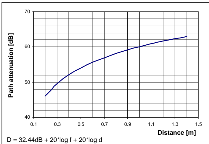
Fig. 12: Power attenuation over distance @24GHz
