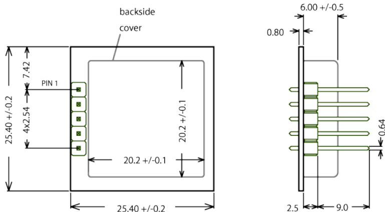
Fig. 4: Mechanical data
