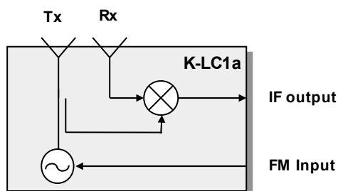
Fig. 1: Block diagram
